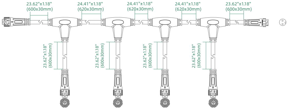
North America version Dimming T-shape junction cable, 2pin, 1 sub-5 dimming interconnection cable, totally 10.17'(380-A-0008) Europe version Dimming T-shape junction cable, 2pin, 1 sub-5 dimming interconnection cable, totally 3.1m(380-A-0010)
