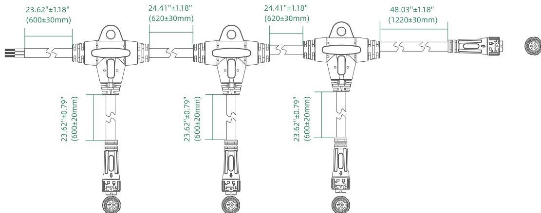
North America version Power T-shape junction cable, 3pin, 1 sub-4 power interconnection cable, totally 10.82'(380-A-0007) Europe version Power T-shape junction cable, 3pin, 1 sub-4 power interconnection cable, totally 3.3m(380-A-0009)
