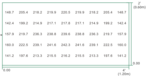
9pcs 315-0008 are installed in a 12'x2'(3.6mx0.6m) cultivation area, the PAR distribution of 3pcs in the middle area 4'x2'(1.2mx0.6m) is shown as:
