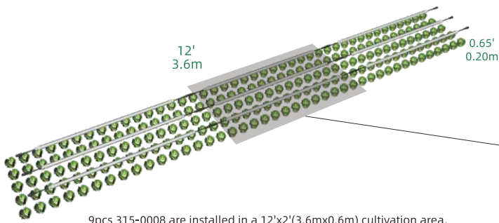
9pcs 315-0008 are installed in a 12'x2'(3.6mx0.6m) cultivation area, the PAR distribution of 3pcs in the middle area 4'x2'(1.2mx0.6m) is shown as:
