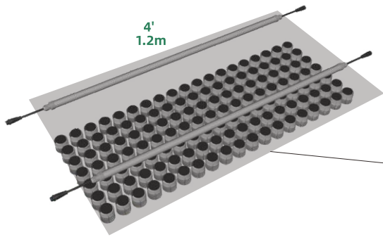
This map displays PAR distribution in an area of 4'x2'(1.2mx0.6m). The distance between the lights and the plants is 0.98'(0.30m), and 2pcs 315-0007 are needed in the planting area of 4'x2'(1.2mx0.6m).
